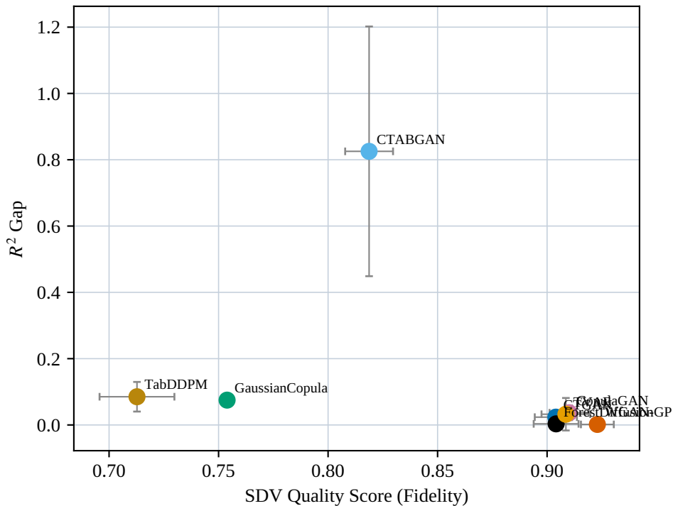
Air Quality: SDV Quality Score (Fidelity) vs R^2 Gap
